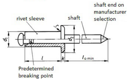
Form A Flathead
