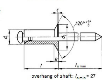
Form B Countersunk head
